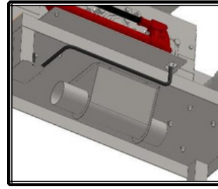
Adaptable discharge made to accept flex auger, rigid auger or even an extended stand to allow for filling bags by hand.
